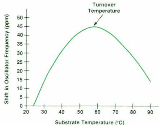
Fig. 2. Frequency shift versus temperature for a crystal. The point where the shift reverses direction is called the turnover temperature.
