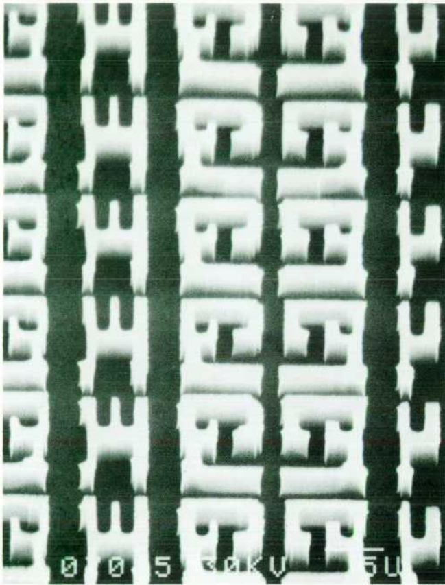
Fig. 9. This is a scanning electron micrograph of the isolation level for a portion of a random-access memory (RAM) patterned in the bottom layer of a trilayer resist structure. The top layer was exposed in the HP electron beam lithography system. The multilayer process reduces proximity effect and gives high-aspect-ratio lines ideal for masking dry etch processes. The smallest critical dimensions shown are 1\ \mu\text{m} .
