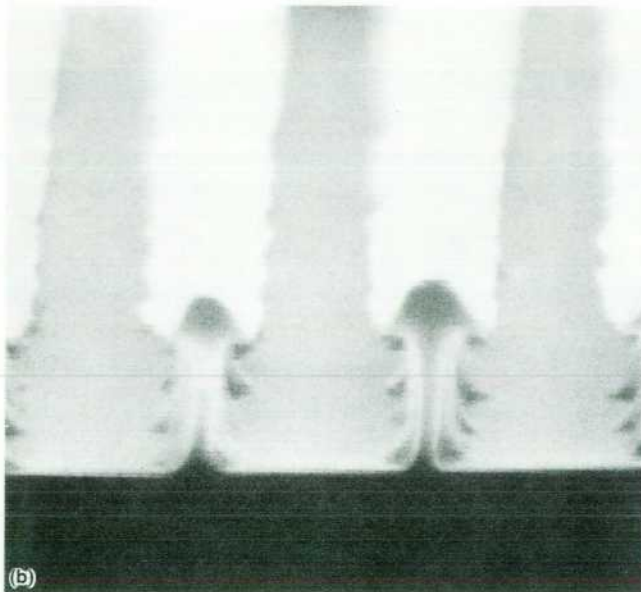
Fig. 11. Mushroom-shaped lift-off structures can be generated by using a two-layer process where the developer for each layer does not affect the other layer. The bottom layer is overdeveloped, creating the undercut profile modeled in (a) for 0.5- \mu\text{m} -wide lines and spaces using a 0.3- \mu\text{m} -thick bottom layer and a 0.1- \mu\text{m} -thick top layer. (b) SEM photograph of the experimental result.
