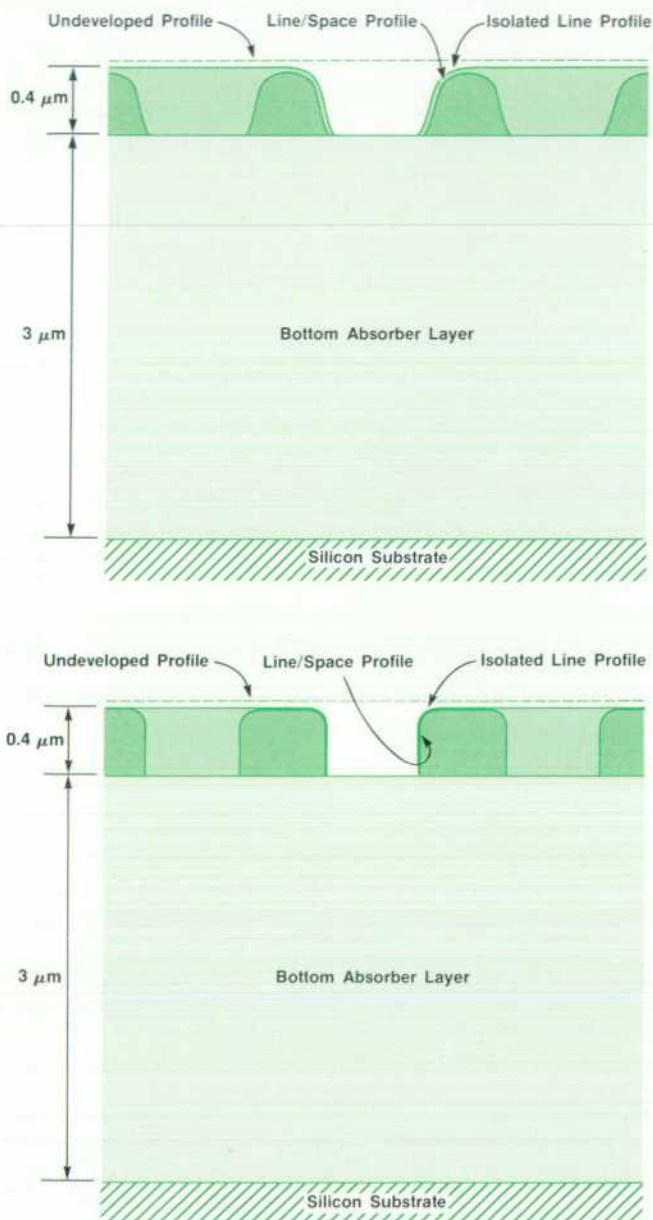
Fig. 7. Proximity effect reduction for lines exposed under the same conditions as for Figs. 2 and 4 except that a 3- \mu\text{m} -thick absorbing polymer layer is used under the 0.4- \mu\text{m} -thick resist layer. Shown are modeled profiles of the developed resist for the central region of five 0.5- \mu\text{m} -wide lines with 0.5- \mu\text{m} -wide spacing and an isolated 0.5- \mu\text{m} -wide line. (a) Beam diameter 0.5 \mu\text{m} . (b) Beam diameter 0.3 \mu\text{m} .
