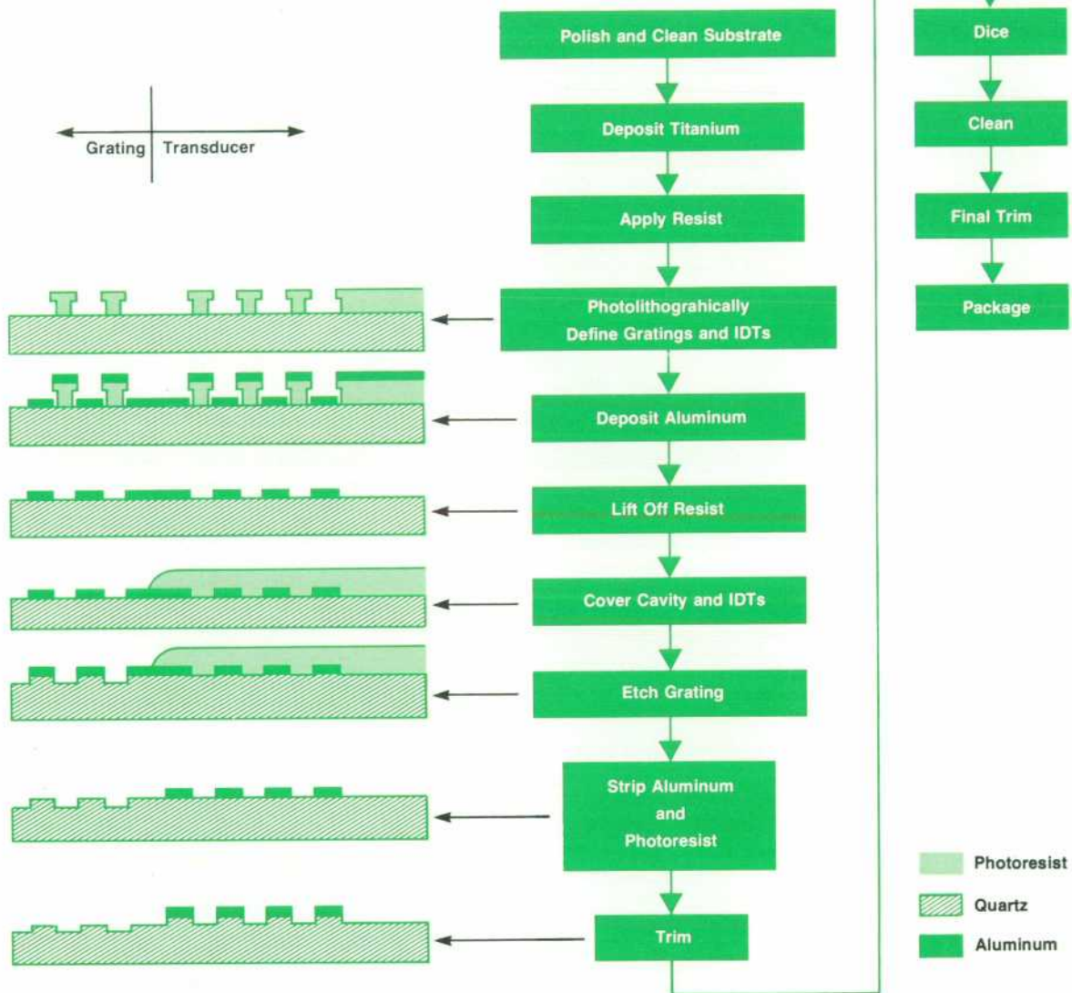
Fig. 1. Fabrication process for SAW resonators.
