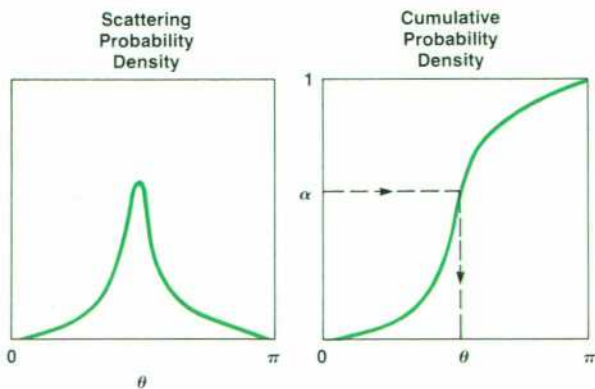
Fig. 1. If scattering angles occur randomly according to the probability density (a), their cumulative distribution is (b), and each angle can be made to correspond to a random number \alpha as indicated. In computer simulations with a random number generator, scattering according to (a) will be simulated.
