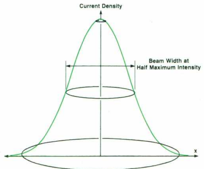
Fig. 4. Gaussian electron beam current density profile showing how beam diameter is defined.
