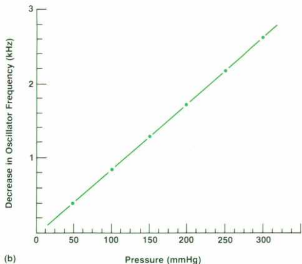
Fig. 6. (a) Physical configuration of pressure sensor using a SAW resonator. (b) Change in resonant frequency versus pressure for sensor shown in (a).
