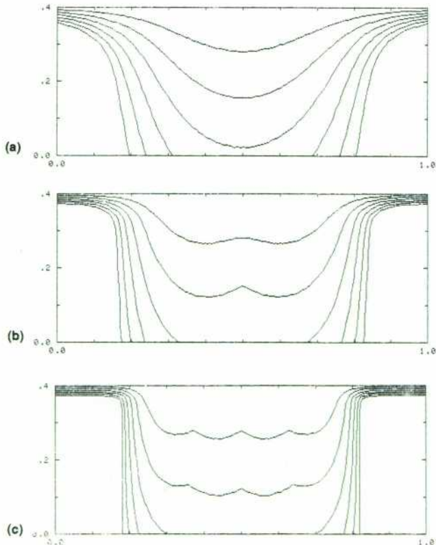
Fig. 3. Modeling data for resist profiles at 25-second intervals during development for a 0.5- \mu\text{m} -wide isolated line exposed with (a) one scan of a 0.5- \mu\text{m} -diameter beam, (b) two adjacent scans of a 0.25- \mu\text{m} -diameter beam, and (c) four adjacent scans of a 0.125- \mu\text{m} -diameter beam.
