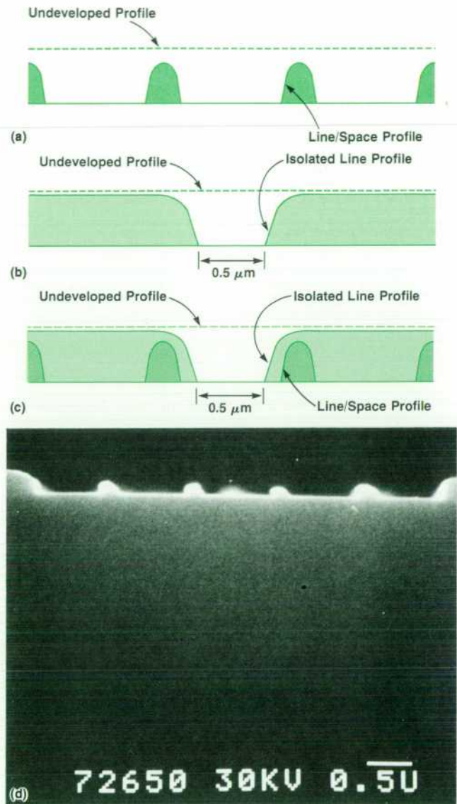
Fig. 2. Proximity effect for lines exposed with a single scan of a 0.5- \mu\text{m} -diameter beam into a 0.4- \mu\text{m} -thick layer of PMMA resist on a silicon substrate. The pixel width is 0.5 \mu\text{m} . Shown are modeled profiles of the developed resist for (a) the central region of five 0.5- \mu\text{m} -wide lines with 0.5- \mu\text{m} -wide spacing and (b) an isolated 0.5- \mu\text{m} -wide line. (c) shows (a) and (b) superimposed for comparison. (d) SEM photograph of experimental result for five equal lines and spaces in PMMA.
