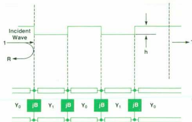
Fig. 3. Equivalent circuit model for a grating reflector.
