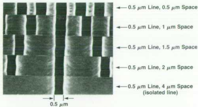
Fig. 8. Proximity effect reduction using multilayer technique. The SEM photographs show the actual widths of 0.5- \mu\text{m} -wide lines as the spacing between the lines is varied from 0.5 \mu\text{m} to 1.0 \mu\text{m} , 1.5 \mu\text{m} , 2.0 \mu\text{m} , and 4.0 \mu\text{m} . The multilayer structure consists of the patterned layer (0.4- \mu\text{m} -thick layer of PMMA resist), the transfer layer (0.07- \mu\text{m} -thick silicon film), and the absorber layer (3- \mu\text{m} -thick layer of Hunt HPR resist). The beam diameter in this experiment was equal to the pixel width.
